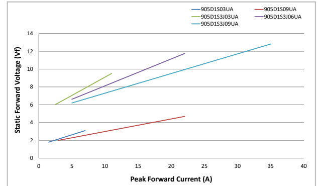
Figure 6a: Static Forward Voltage vs. Current
