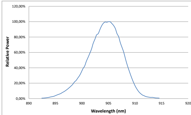
Figure 5: Typical Spectral Plot
